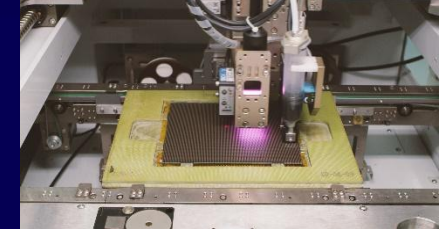
Lamp board Inkjet
